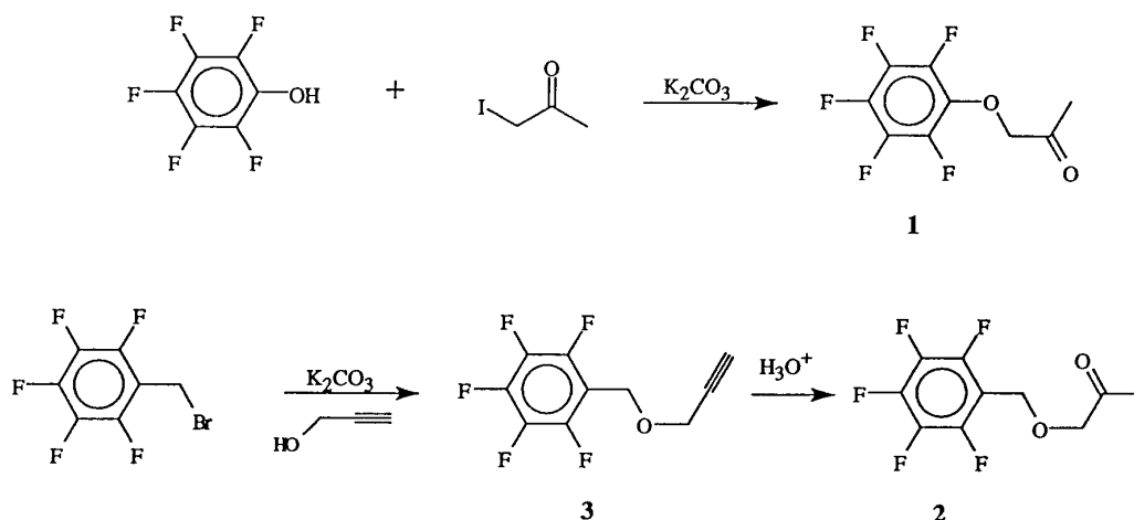
Figure 1. Synthesis of 1 and 2.
